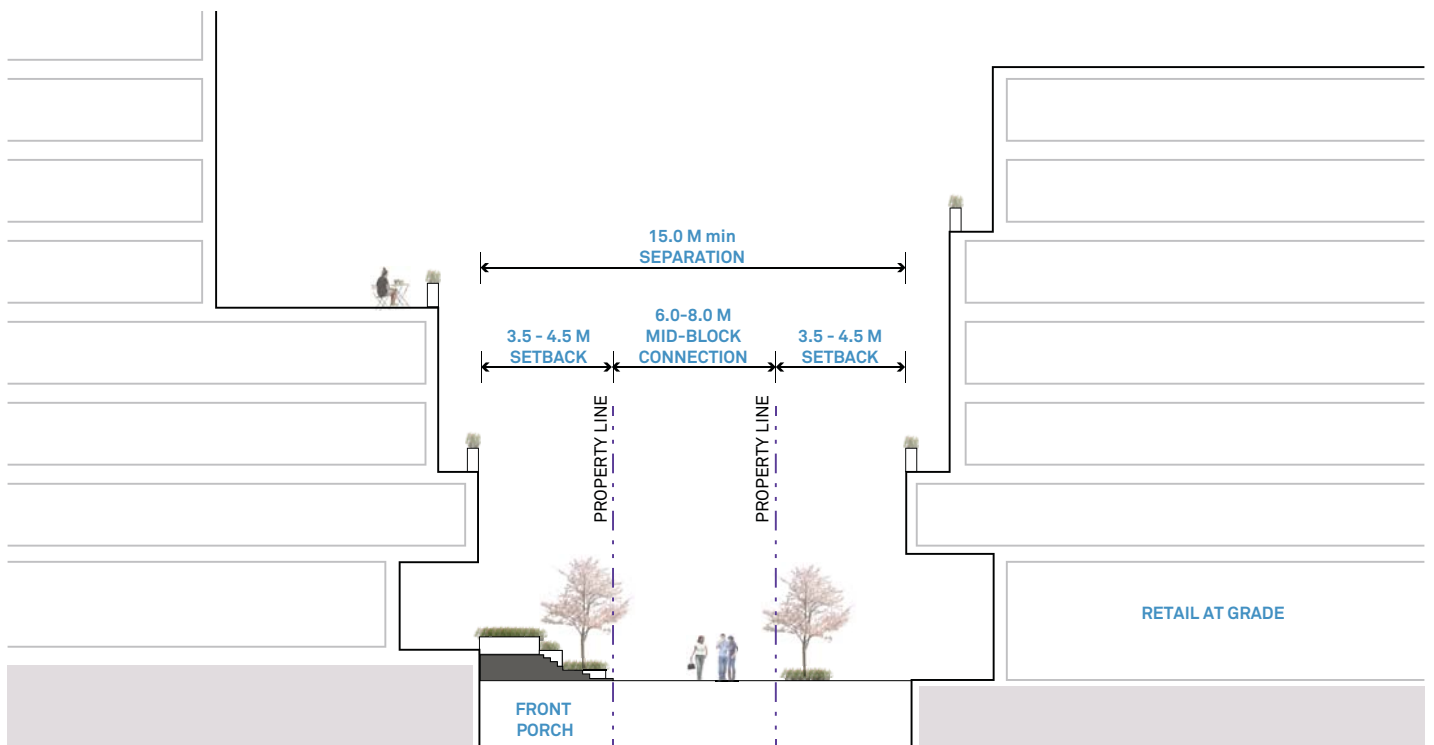
Pedestrian meadows between buildings with active frontages and ground floor residential entrances. See Performance Standard 5.3.7 for separation distances between buildings above the 6th storey.
