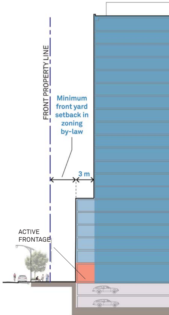
Envelope Performance Standards for Podium at 6-storays.
