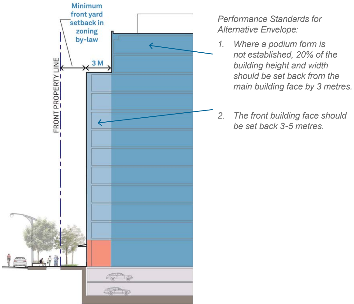
Performance standards for Mid-Rise buildings not located on intensification corridors.
