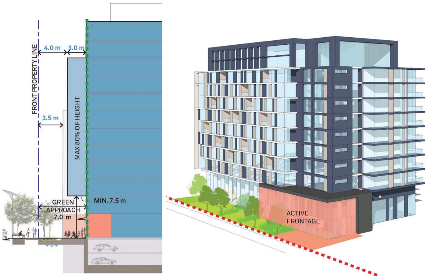
On Intensification Corridors, Mid-Rise buildings should establish a 7 metre wide front yard Green Approach. Projections and cantilevers are permitted to extend this area above 7.5 metres.
