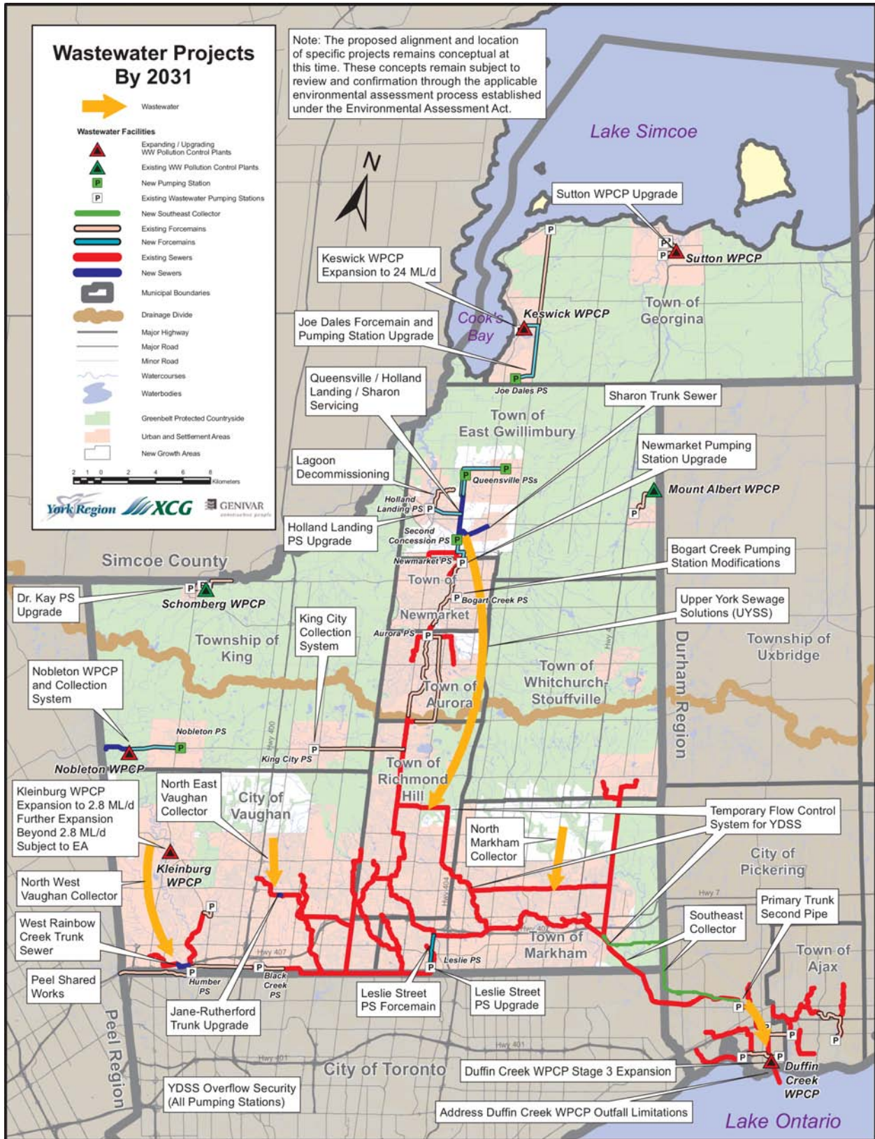
Figure 5-2 York Region Wastewater Servicing by 2031.
